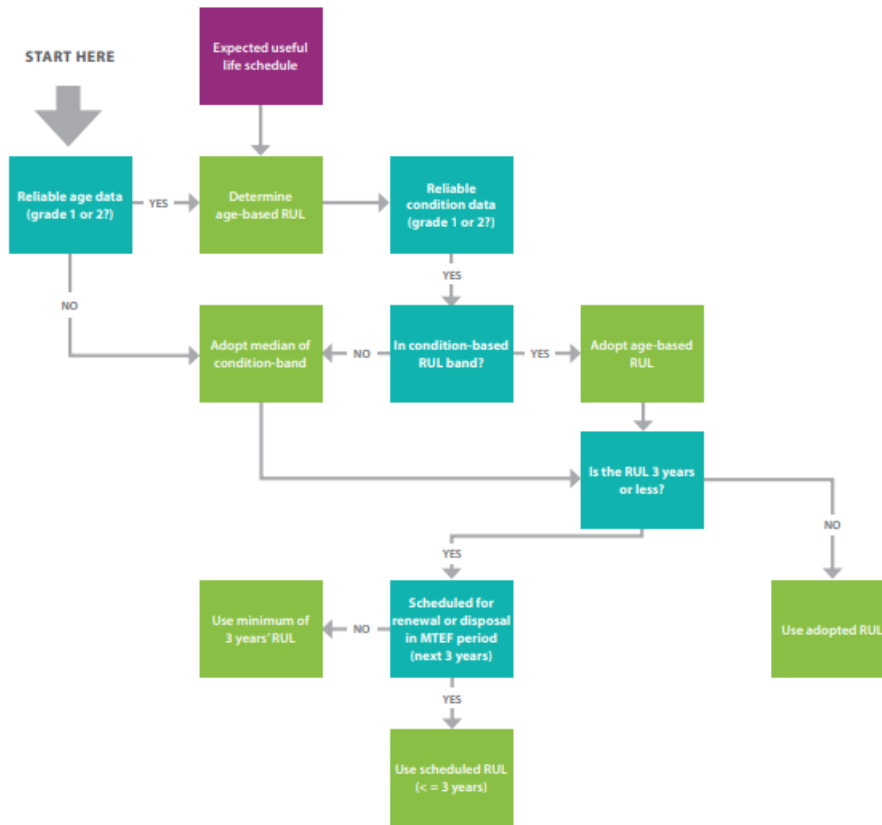
FIGURE 3.16: RUL algorithm
